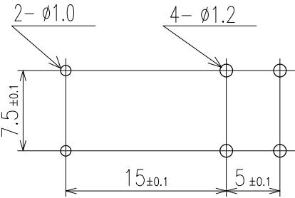
DRILLING DIAGRAM?BOTTM VIEW?
